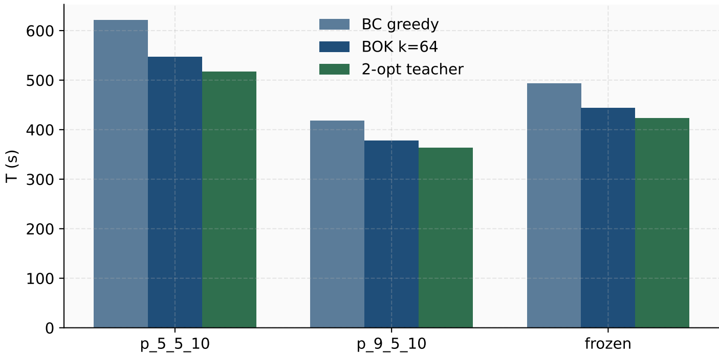
Held-out / frozen profiles — BC vs sampling vs teacher
