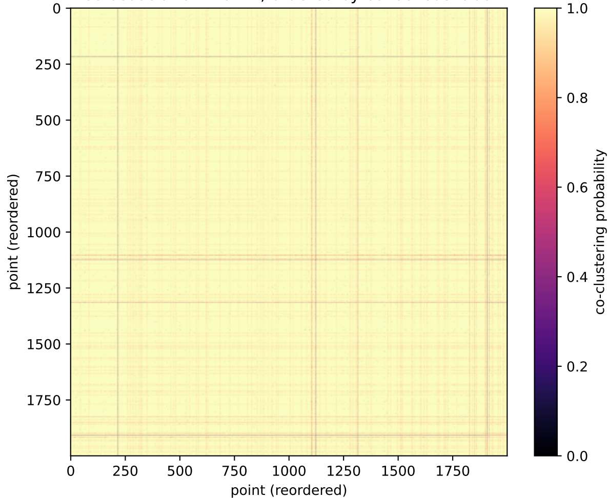
Co-association matrix, ordered by consensus label
