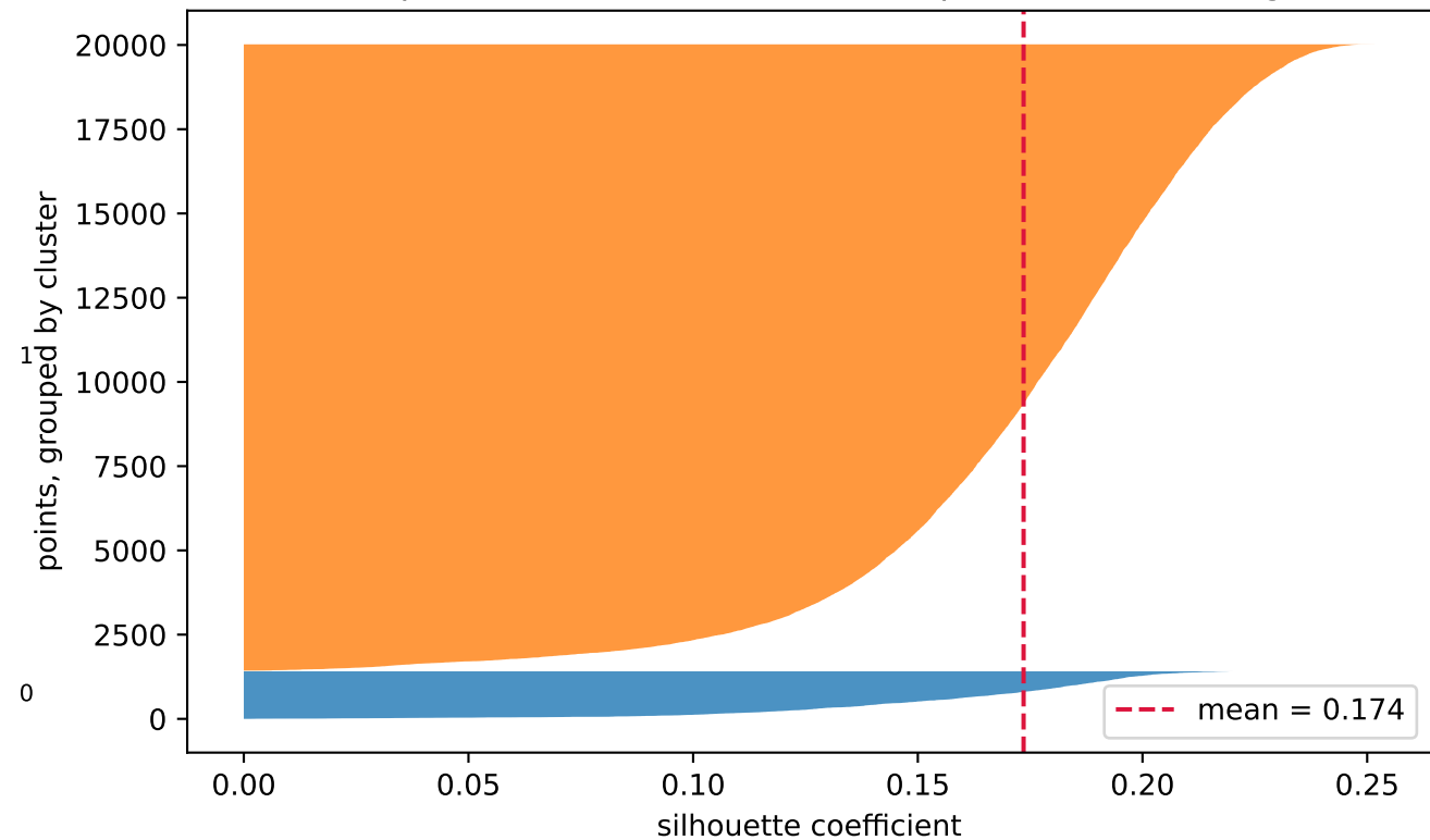
Per-point silhouette distribution — preferred clustering
