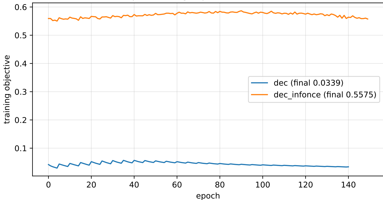
Deep clustering objectives (brief §4.1.1)
