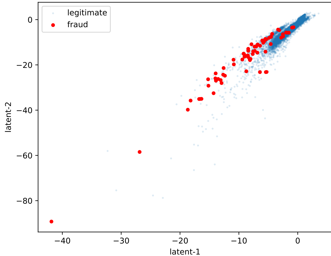
Same space — held-out Class overlay
