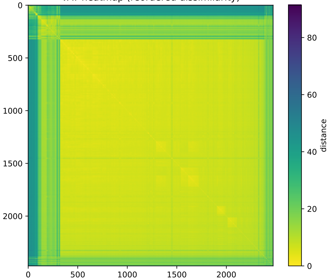
VAT heatmap (reordered dissimilarity)
