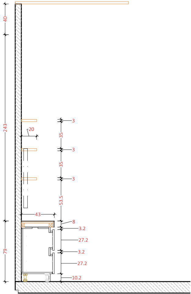
Side Section
