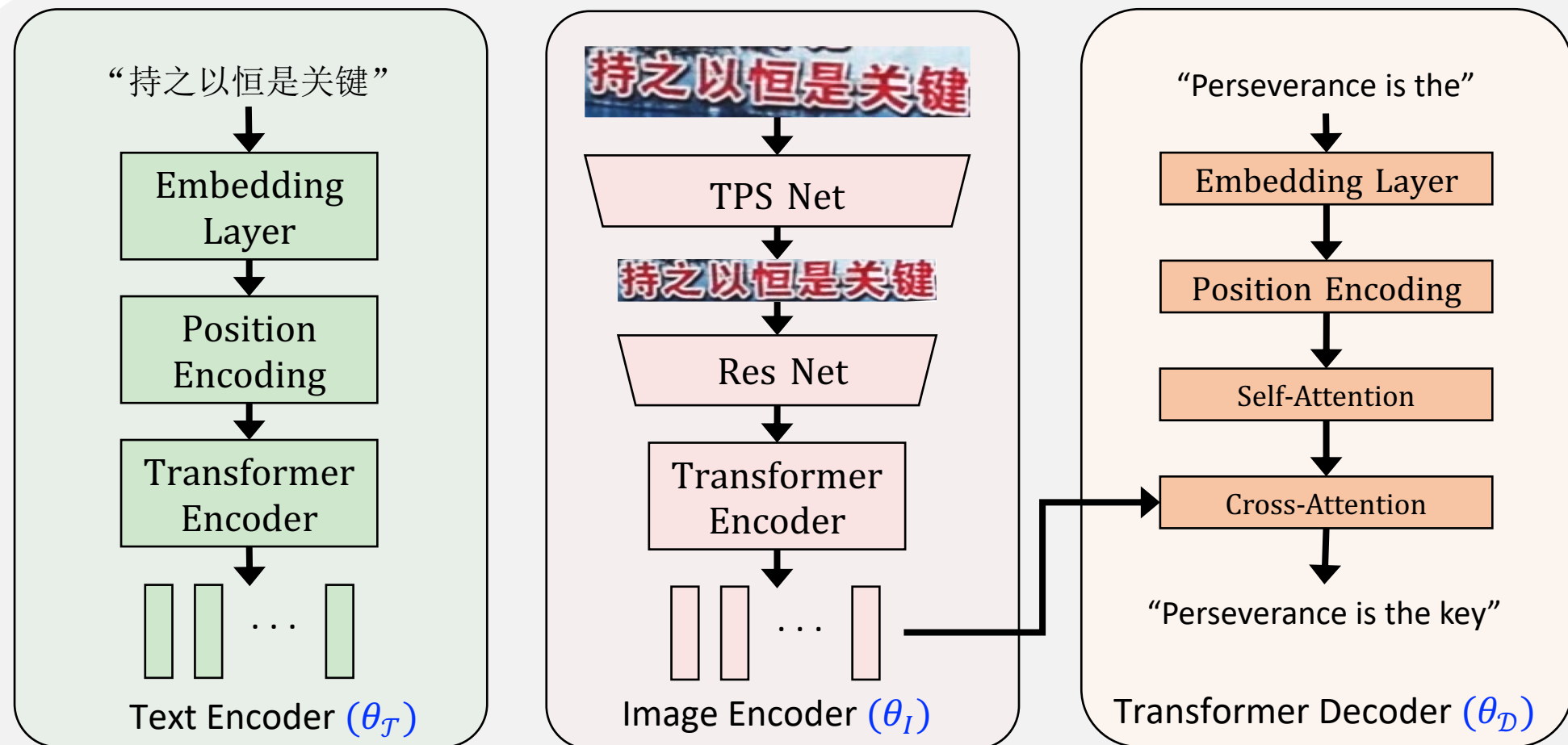
(b) Architecture of text encoder, image encoder, and transformer decoder.
