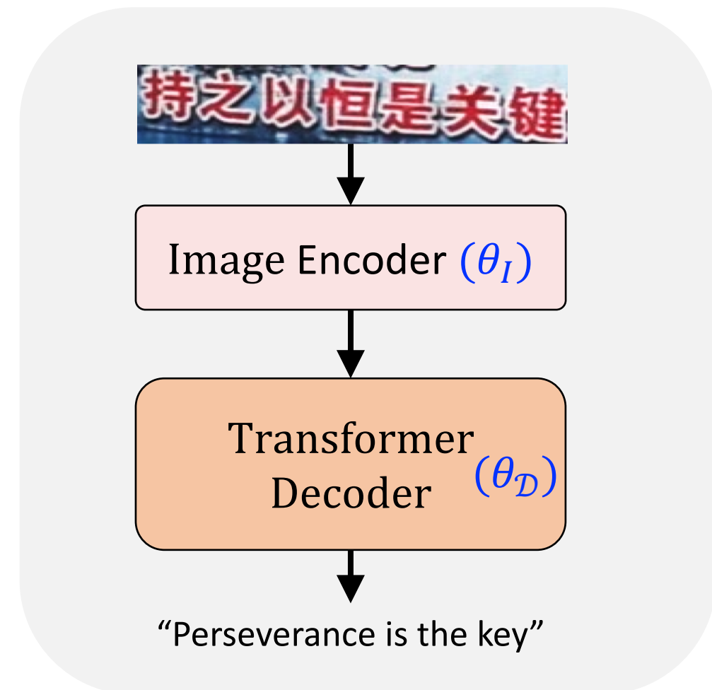
(c) Workflow of text image translation during evaluation.
