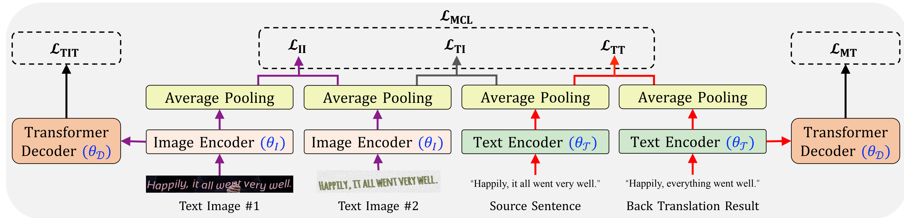
(a) Workflow of model training with modal contrastive loss and text image translation loss.
