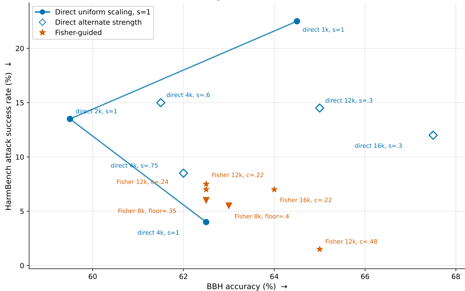
Direct versus Fisher-guided first-cue Grad interventions
