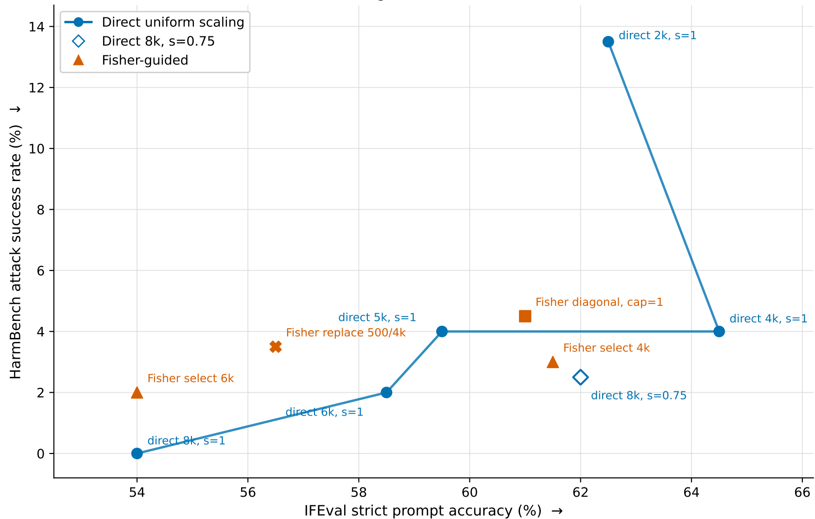
Direct versus Fisher-guided first-cue Grad interventions
