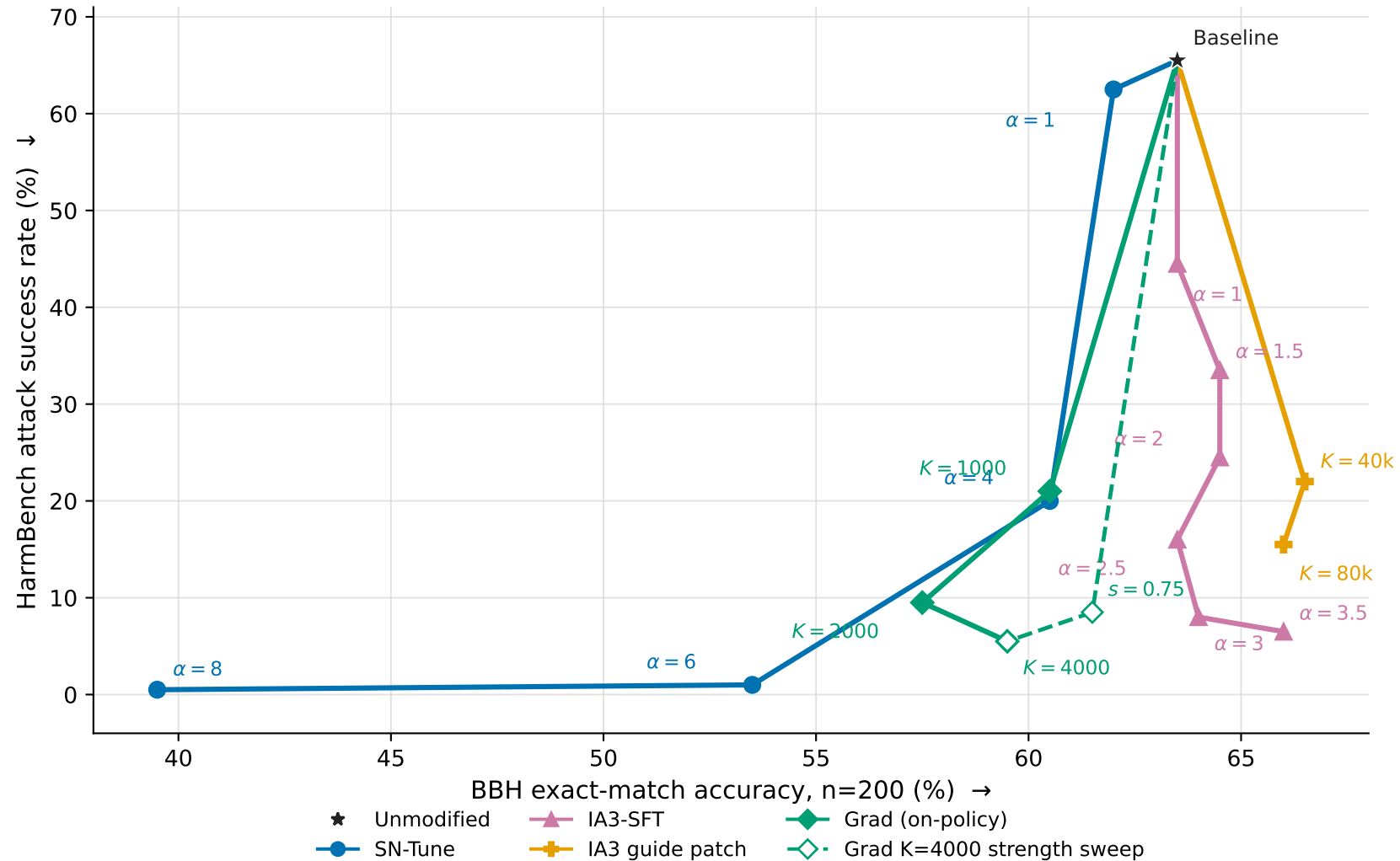
Main safety-BBH trajectories Grad: solid K sweep at s=1 ; dashed K=4000 strength sweep
