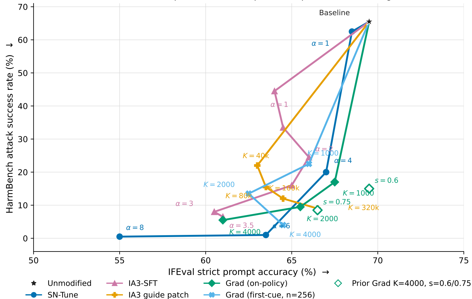
Main safety-instruction-following trajectories Grad: solid K sweeps at s=1 ; hollow points are prior K=4000 strengths
