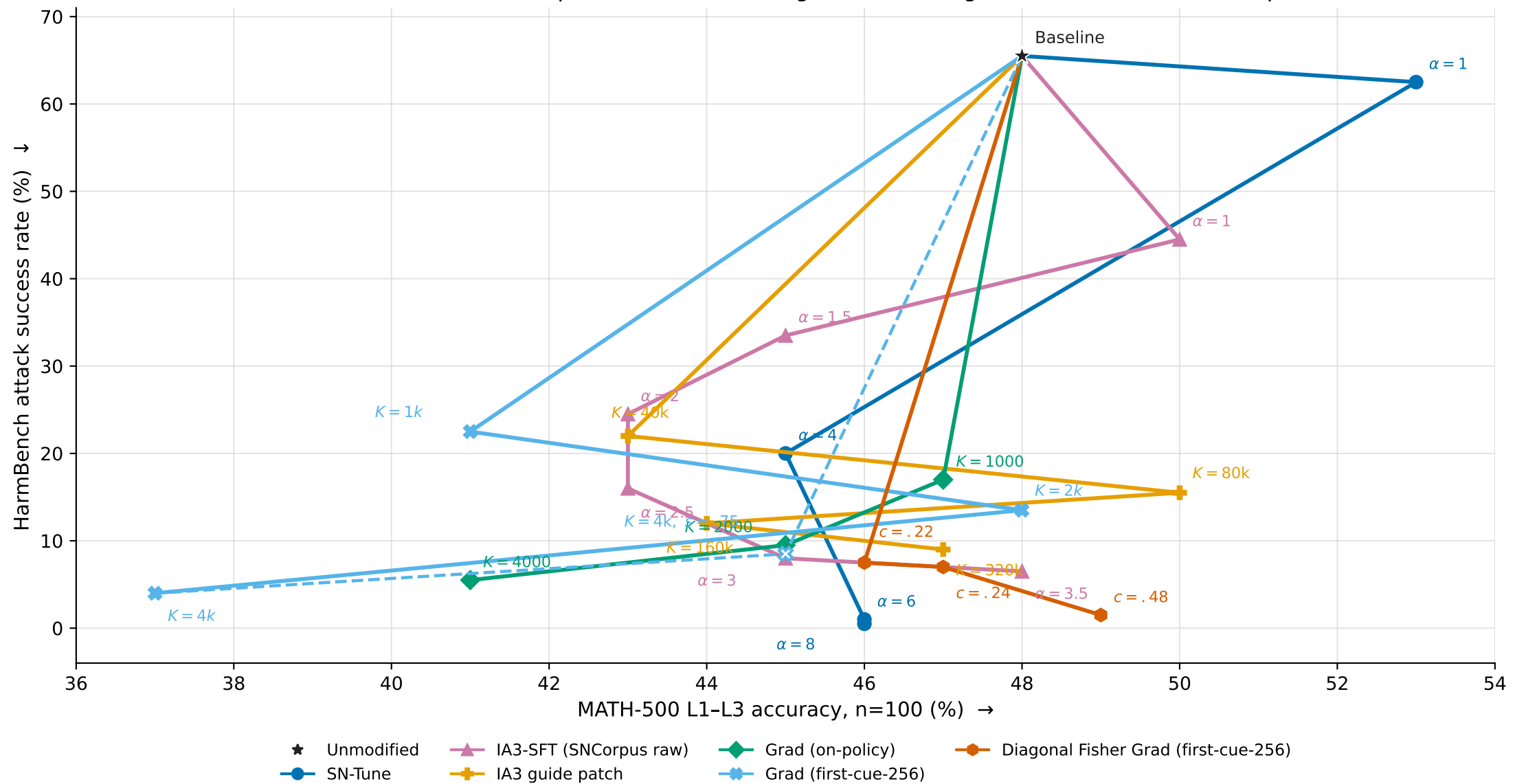
Safety-math trade-offs Direct: solid s=1 K sweep, dashed K=4k strength branch; diagonal Fisher: K=12k c sweep
