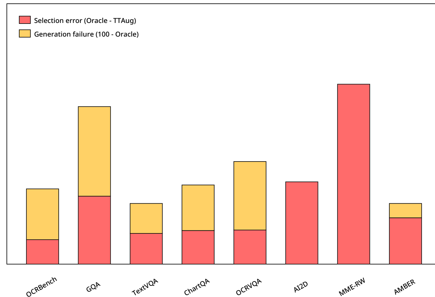
(b) TTAug error decomposition
