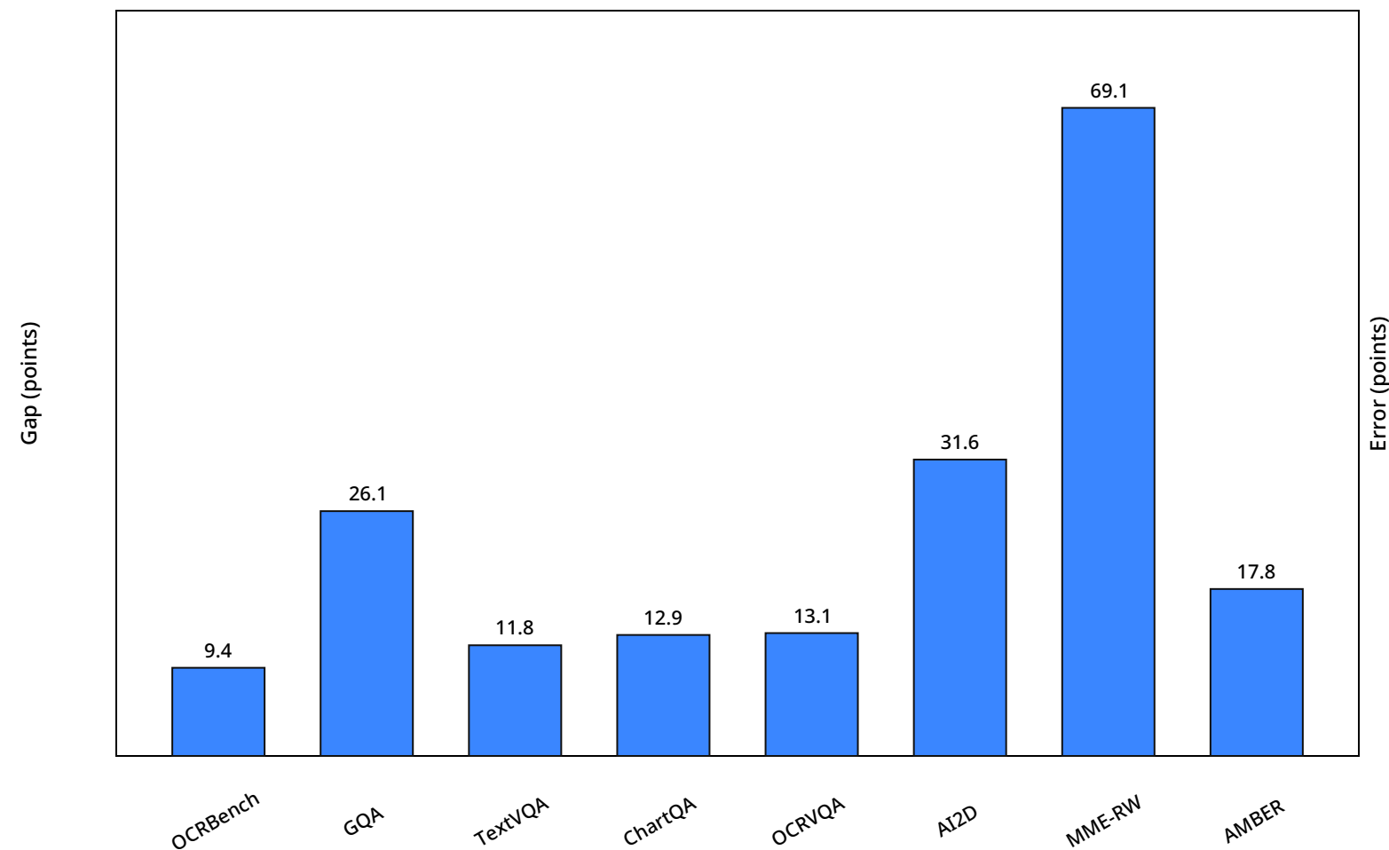
(a) Oracle--TTAug gap
