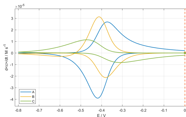
Figure 2 — Stagnant layer of 200 \mu\text{m} , A + e = B followed by B \rightarrow C ( k = 0.05 \text{ s}^{-1} ), 10 mV/s: derivative of the mean concentration of A, B and C over the layer.
