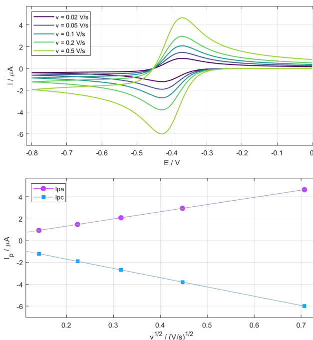
Figure 1 — Fast couple ( k^0 = 1 cm/s), five scan rates from 0.02 to 0.5 V/s: voltammograms and the lines I_p = f(v^{1/2}) drawn by the Series window.
