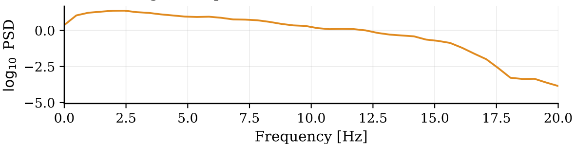
(c) After \log_{10} compression
