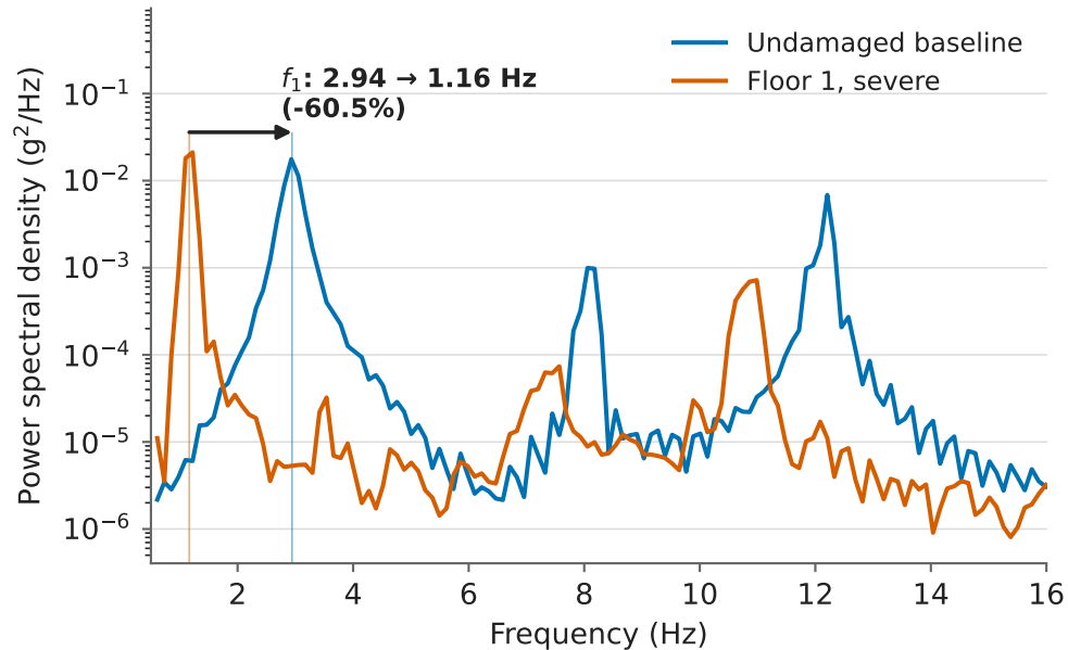
(a) The fundamental migrates under damage
