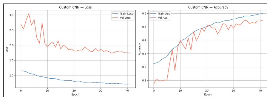
Figure 2: Custom CNN — training and validation loss and accuracy curves.
