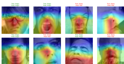
Figure 7: Grad-CAM heatmaps for 8 test images, showing the regions of the face that ResNet-18 attended to for each prediction.
