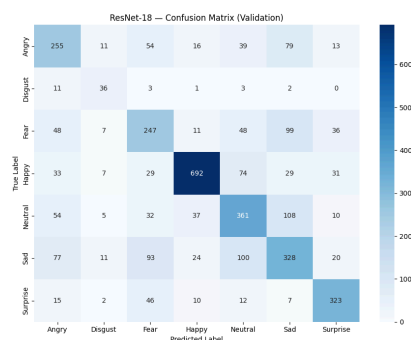
Figure 5: ResNet-18 confusion matrix on the validation set.
