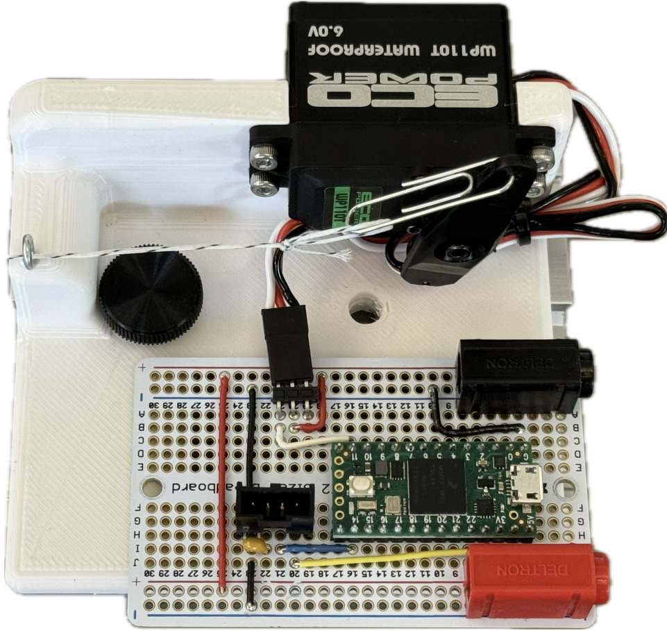
FIG. 3. A photo of the completed device, showing the circuitboard, servo (EcoPower WP110T), and routing of the drive string.
