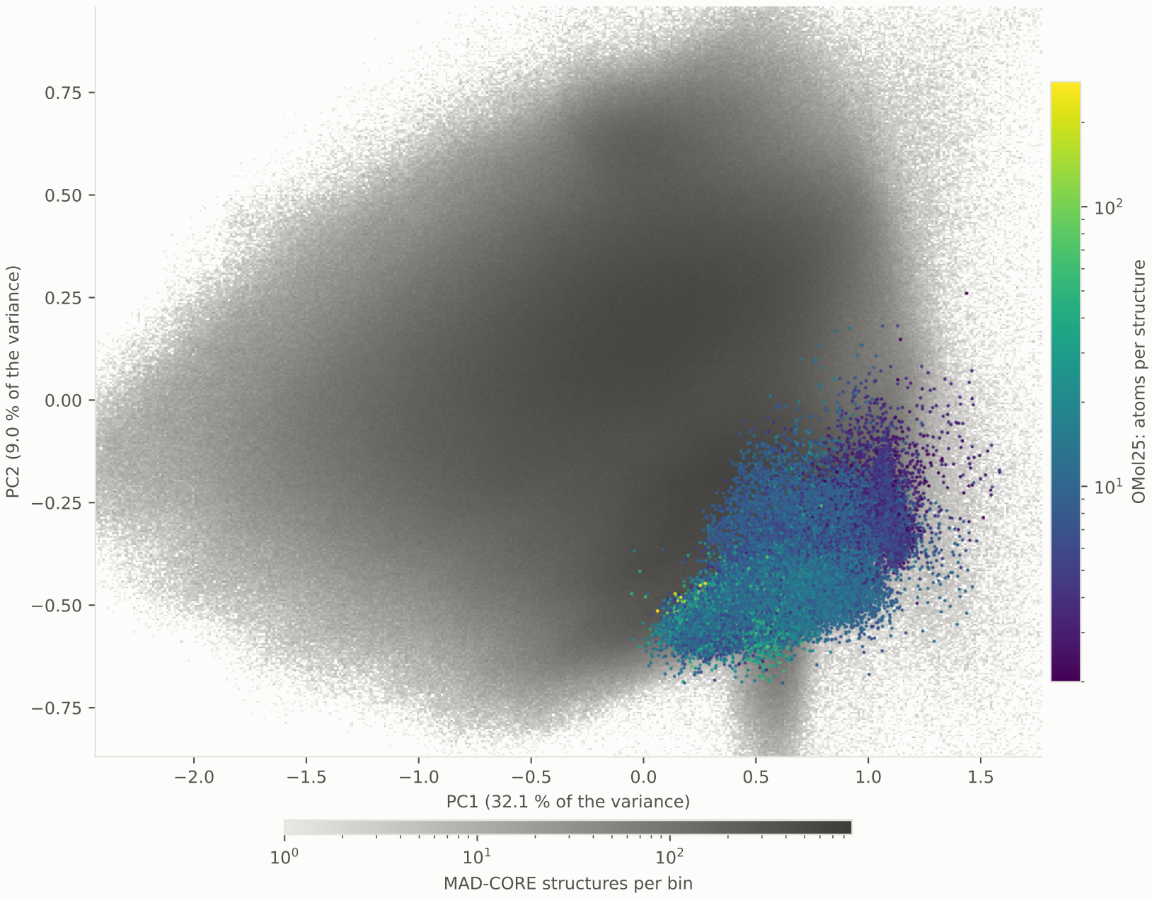
MAD-CORE feature PCA, fitted on all 16,777,216 structures (grey) OMol25: 367,234 structures, 100,000 drawn (colour)
