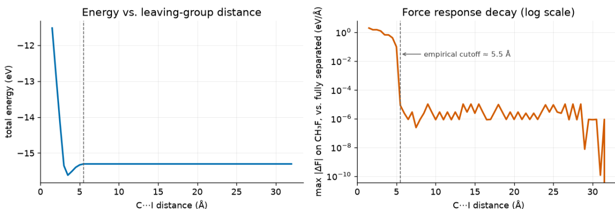
Reaction-coordinate scan: SN2 -- matched BPNN + dipole
