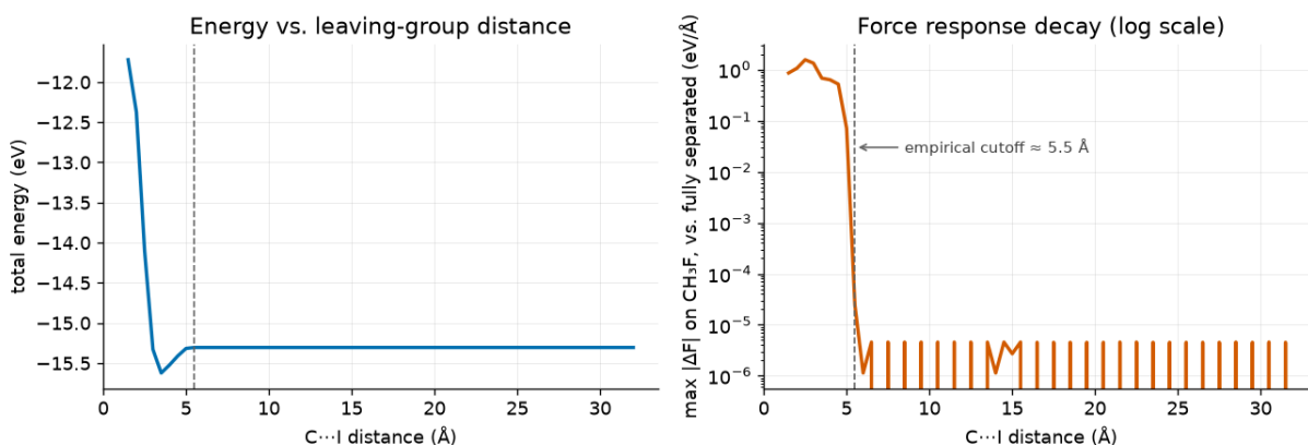
Reaction-coordinate scan: SN2 -- matched BPNN + dipole (v2)
