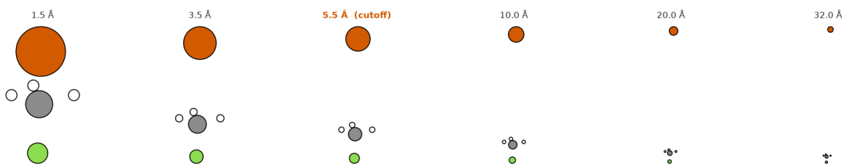
CH 3 F...I - geometry along the scan -- SN2 -- matched BPNN + dipole (v2)
