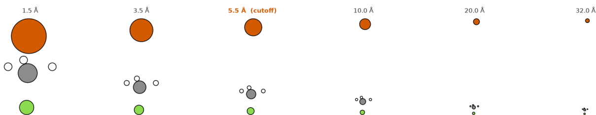
CH 3 F...I - geometry along the scan -- SN2 -- matched BPNN + dipole (v3)
