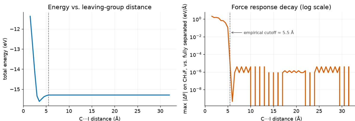
Reaction-coordinate scan: SN2 -- matched BPNN + dipole (v3)
