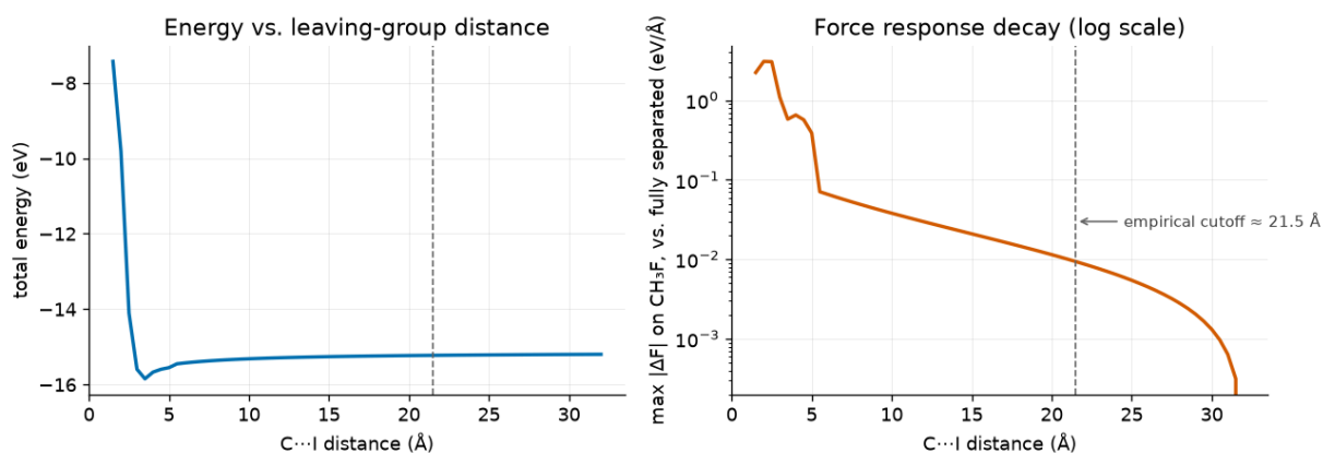
Reaction-coordinate scan: SN2 -- matched LOREM
