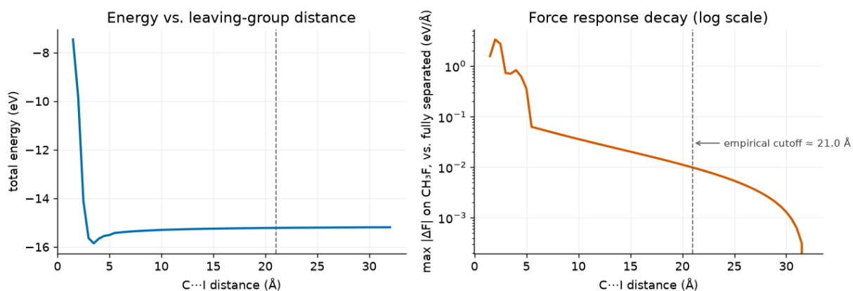
Reaction-coordinate scan: SN2 -- matched LOREM + dipole
