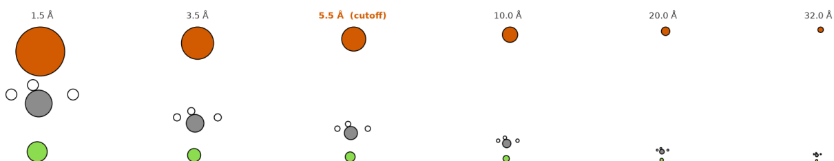
CH 3 F...I - geometry along the scan -- SN2 -- matched PET + dipole
