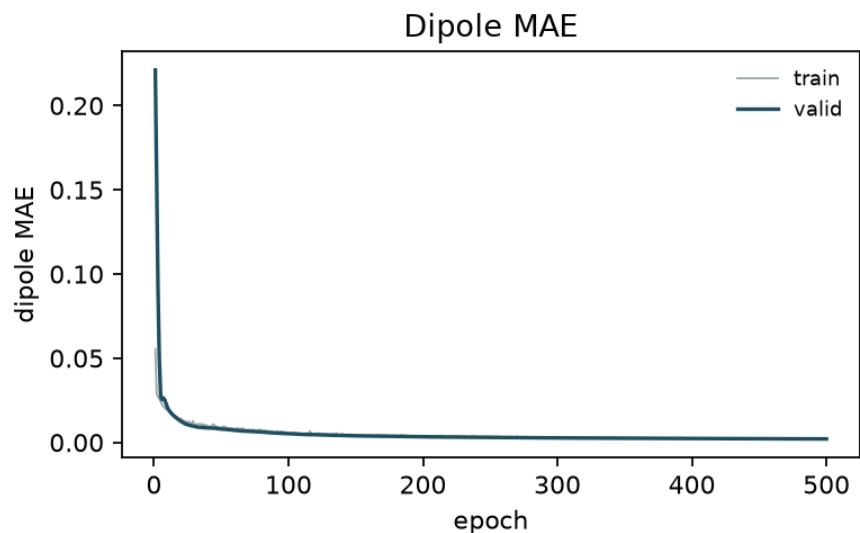
Figure S1: Dipole MAE versus epoch for the hybrid + LJ-scale Menshutkin run (companion to Figure 5).
