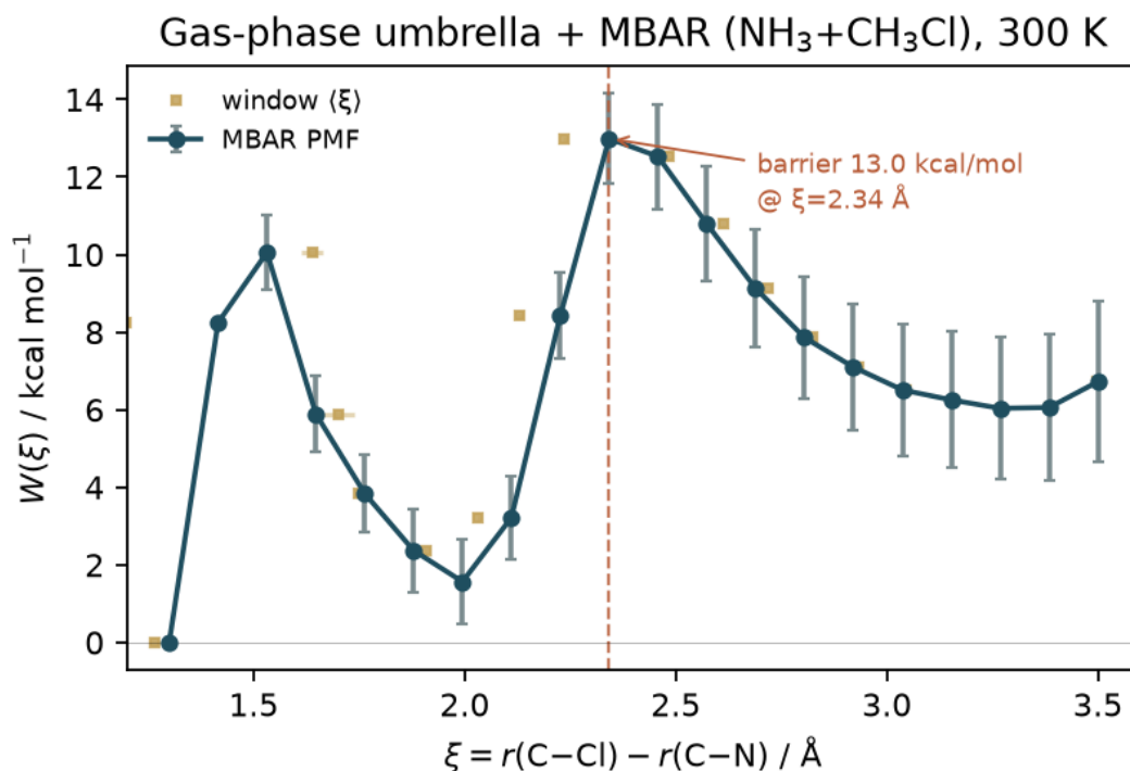
Figure 9: Gas-phase umbrella + MBAR PMF for \text{NH}_3 + \text{CH}_3\text{Cl} along \xi = r(\text{C}-\text{Cl}) - r(\text{C}-\text{N}) at 300 K (20 windows; source artifacts/umbrella/ ).
