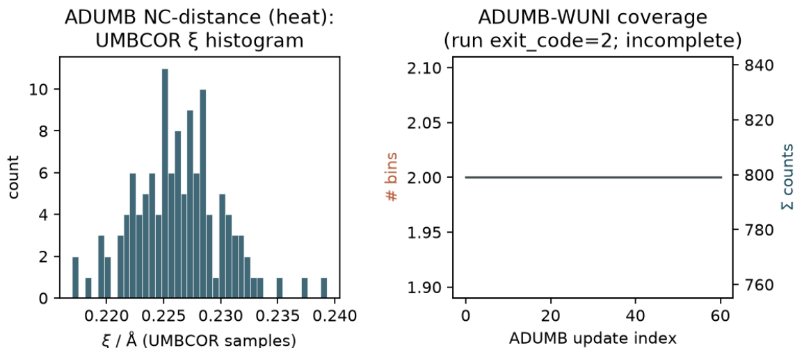
Figure 10: CHARMM ADUMB status for the NC-distance Menshutkin setup ( artifacts/nh3_ch3cl/adumb_nc_distance/ ): UMBCOR \xi histogram during heat (left) and ADUMB-WUNI bin coverage versus update index (right). The run did not finish cleanly ( exit_code=2 ); no WHAM barrier is claimed.
