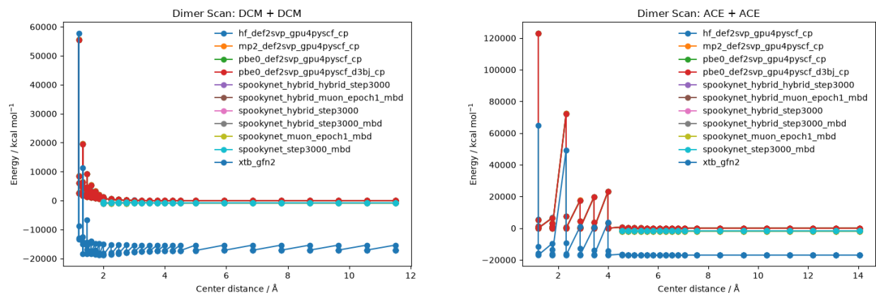
Figure 7: Rigid dimer interaction scans for DCM–DCM (left) and ACE–ACE (right) from the dimer-scan campaign ( scan_results_clean.csv ). Energies are interaction values relative to separated monomers.
