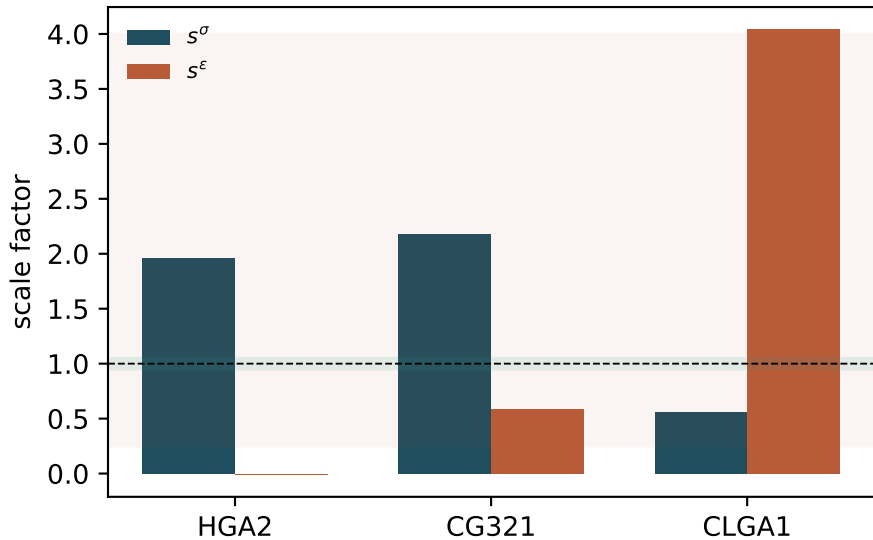
Learned LJ scales (3 types moved)
