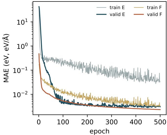
Energy & force MAE
