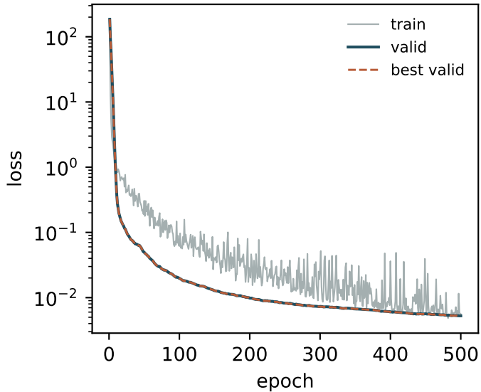
Hybrid MM + LJ-scale training
