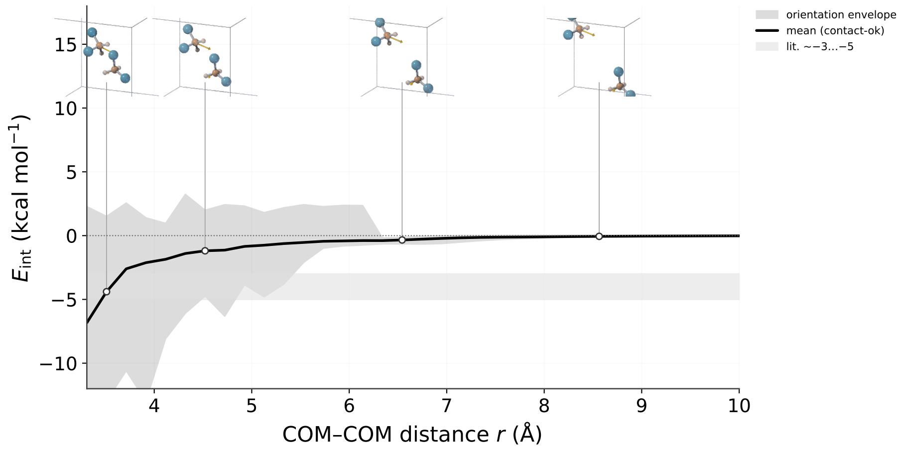
DCM-DCM contact-ok profile — atoms by crameri:vik charge (ray d5 q3)
