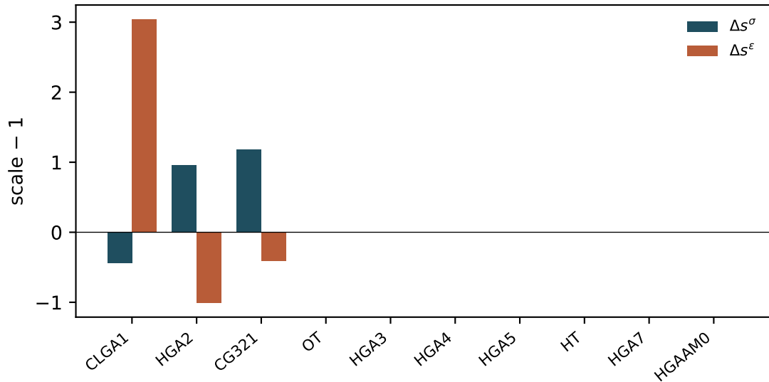
Largest LJ-scale deviations from 1
