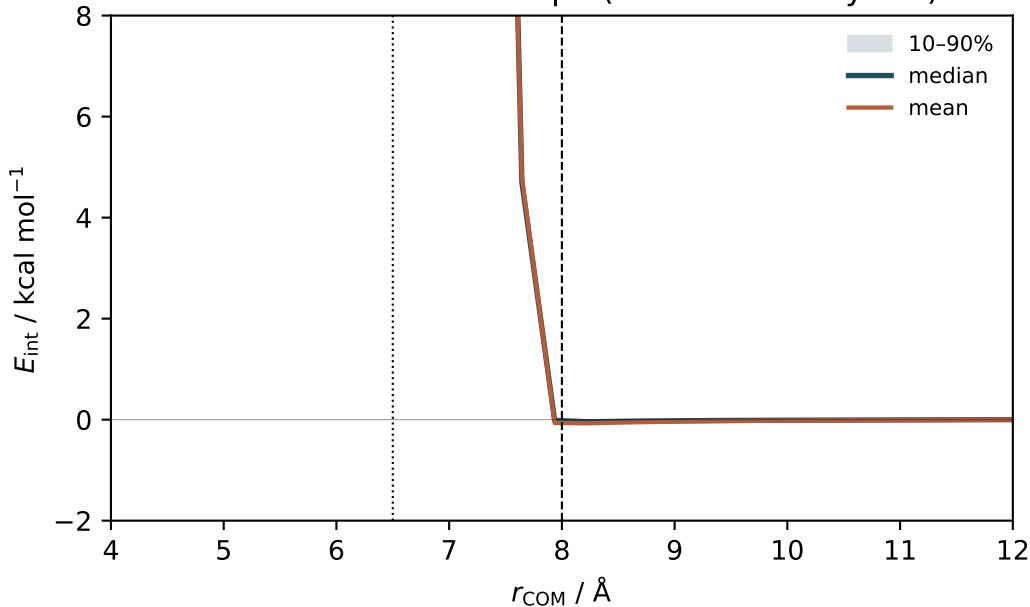
ACE orientation envelope (DCM-trained hybrid)
