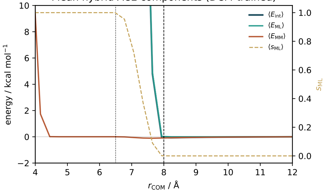
Mean hybrid ACE components (DCM-trained)
