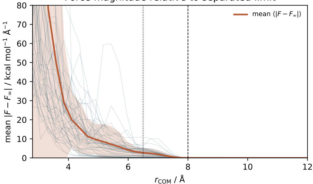
Force magnitude relative to separated limit
