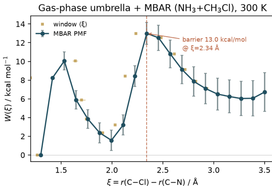
Figure 11: Gas-phase umbrella + MBAR PMF for \text{NH}_3+\text{CH}_3\text{Cl} along \xi = r(\text{C}-\text{Cl})-r(\text{C}-\text{N}) at 300 K (20 windows; source artifacts/umbrella/ ).
