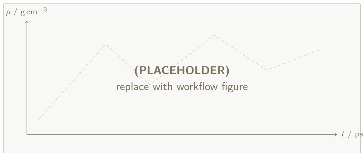
Figure 10: (PLACEHOLDER) Density time series \rho(t) for hybrid DCM and ACO production windows once metrics.json density fields are populated by pbcliquiddensity_dyn .
