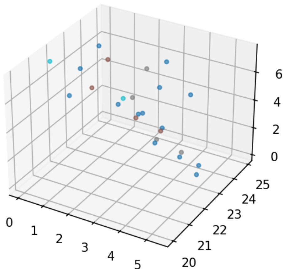
Figure 2: Subset of atoms from pdb/init-packmol.pdb (two BENZ molecules in the default script).
