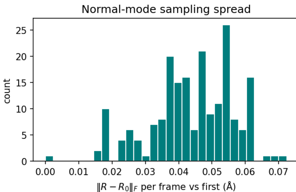
Figure 4: Distribution of displacements relative to the first sampled frame (out/06_sampled.npz).
