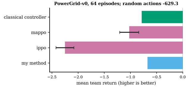
Figure 4. Output of examples/algorithms/baseline_comparison.py: mean return on 64 shared evaluation episodes (seed 1); error bars are the standard deviation over two training seeds.
