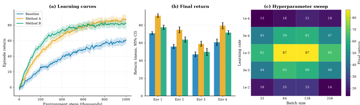
Figure 13.1: A three-panel summary figure made with plotkit ( examples/plotkit_gallery.py , synthetic data): (a) learning curves of three methods over eight seeds with 95 % confidence bands and EMA smoothing, (b) grouped bars with 95 % confidence intervals, (c) an annotated heatmap of a hyperparameter sweep. Each method keeps its Okabe-Ito colour in every panel.
