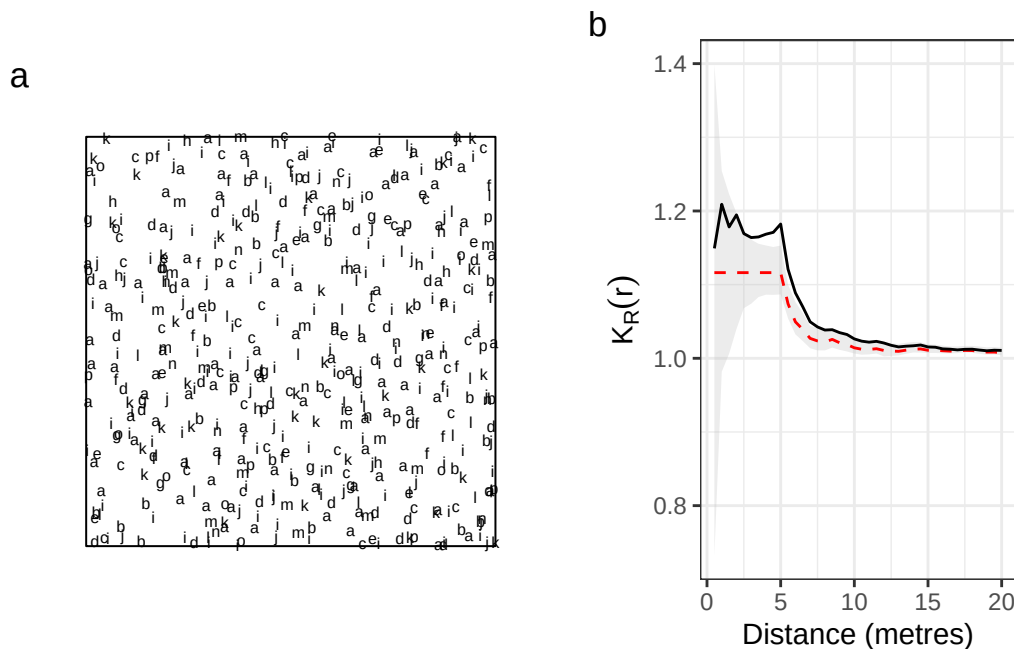
Figure 3. (a) Multitype Strauss point pattern mimicking limiting similarity in a 100x100-m window. The pattern of interaction is obtained using un multi-Strauss inhibition process with a 5-m range and an interaction matrix corresponding to the cophenetic distance matrix derived from the clustered phylogenetic tree. The strength of repulsion between each pair of points decreases with their distance in the phylogeny. (b) K_R(r) computed with the cophenetic between-species distance matrix indicates a significant positive departure from the 1% confidence envelop of the species equivalence hypothesis obtained from 1000 Monte Carlo simulations from 3 to 10 m, with a peak at 5 m: because of competition, the neighbourhood diversity is higher than expected.
