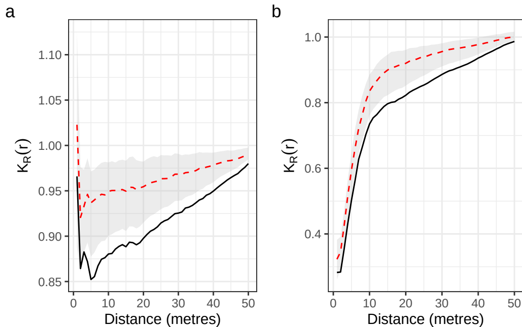
Figure 2. Test of the species equivalence hypothesis of the habitat preference-experiment with (a) a completely random point pattern and (b) a clustered one. The K_R(r) curve (solid line is computed with the cophenetic distance matrix derived from the clustered phylogenetic tree and tested against a 1% confidence envelop of the species equivalence hypothesis obtained from 1000 Monte Carlo simulations (grey area; the dotted line represents the average simulated values). Negative departure from null hypothesis is observed over 2 m: the neighbourhood phylogenetic diversity is below its expected value due to habitat preference.
