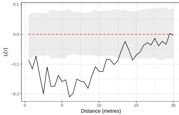
Figure 4. Spatial pattern of Paracou plot 6. Significant (departure from the 1% confidence envelop of complete spatial randomness obtained from 1000 Monte Carlo simulations) repulsion between trees is detected up to 12 m.
