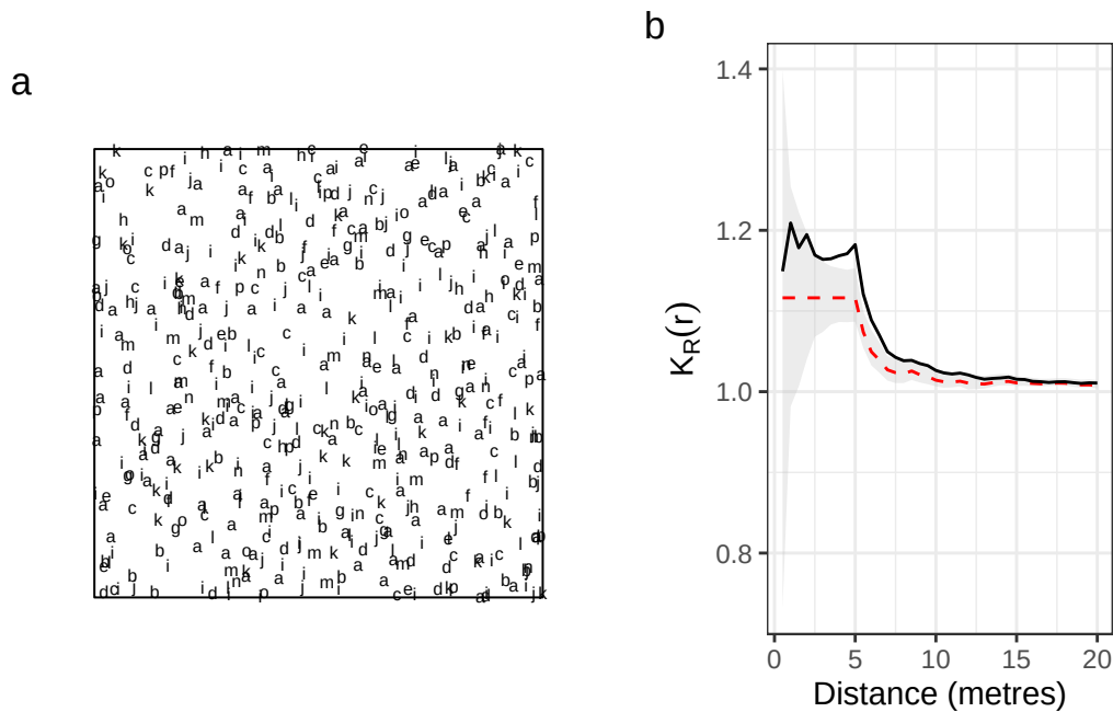
Figure 3. (a) Multitype Strauss point pattern mimicking limited similarity in a 100x100-m window. The pattern of interaction is obtained using un multi-Strauss inhibition process with a 5-m range and an interaction matrix corresponding to the cophenetic distance matrix derived from the clustered phylogenetic tree. (b) K_R(r) computed with the cophenetic between-species distance matrix indicates a significant positive departure from the 1% confidence envelop of the species equivalence hypothesis obtained from 1000 Monte Carlo simulations from 3 to 10 m, with a peak at 5 m: because of competition, the neighbourhood diversity is higher than expected.
