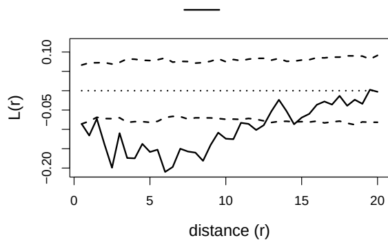
Figure 4. Spatial pattern of Paracou plot 6. Significant (departure from the 1% confidence envelop of complete spatial randomness obtained from 1000 Monte Carlo simulations) repulsion between trees is detected up to 12 m.
