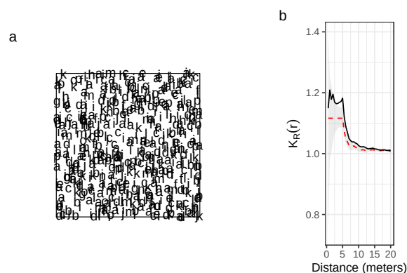
Figure 3. (a) Multitype Strauss point pattern mimicking limited similarity. The pattern of interaction is obtained using un multi-Strauss inhibition process with a 5-m range and an interaction matrix corresponding to the cophenetic distance matrix derived from the clustered phylogenetic tree. The strength of repulsion between each pair of points decreases with their distance in the phylogeny. (b) K_R(r) computed with the cophenetic between-species distance matrix indicates a significant positive departure from the 1% confidence envelop of the species equivalence hypothesis obtained from 1000 Monte Carlo simulations from 3 to 10 m, with a peak at 5 m: because of competition, the neighbourhood diversity is higher than expected.
