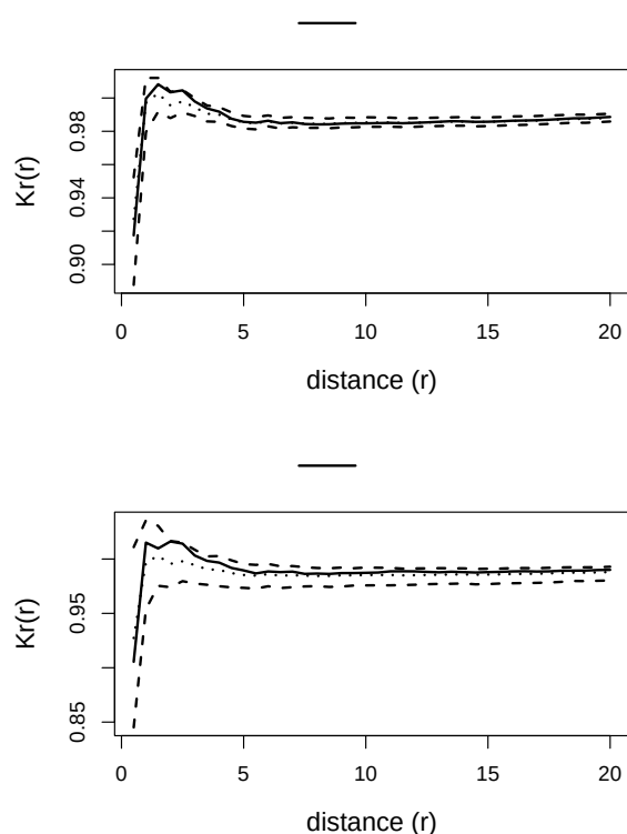
Figure 7. Non-significant positive departure at short distances of the K_R -function applied to Paracou plot 6 considering the phylogenetic and functional distances between species.
