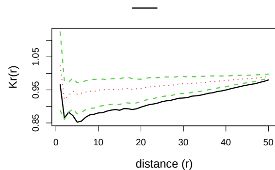
Figure 2. Test of the species equivalence hypothesis of the habitat preference-experiment. The K_R(r) curve (solid line) is computed with the cophenetic distance matrix derived from the clustered phylogenetic tree and tested against a 1% confidence envelop of the species equivalence hypothesis obtained from 1000 Monte Carlo simulations (dashed lines; the dotted line represents the average simulated values). Negative departure from null hypothesis is observed over 2 m: the neighbourhood phylogenetic diversity is below its expected value due to habitat preference.
