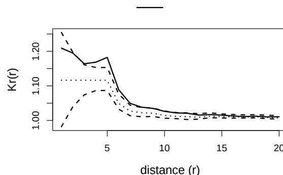
Figure 5. Spatial pattern of competitive interaction between 16 species in a 1-ha plot. The pattern of interaction is obtained using a multi-Strauss inhibition process with a 5 m range and an interaction matrix corresponding to the cophenetic distance matrix derived from the clustered phylogenetic tree. K_R(r) computed with the cophenetic between-species distance matrix indicates a significant positive departure from the 1% confidence envelope of the species equivalence hypothesis obtained from 1000 Monte Carlo simulations from 3 to 9 m.
