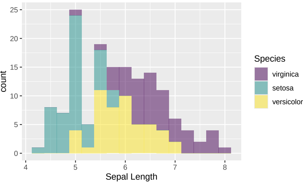
Overlapping Histogram
