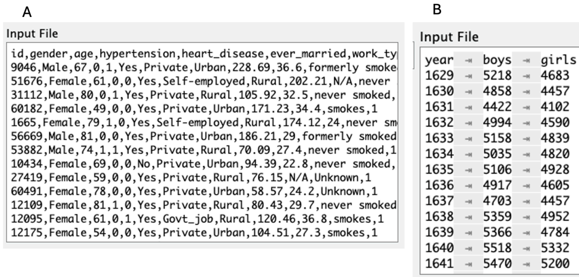
Figure 5.2: File formats.
