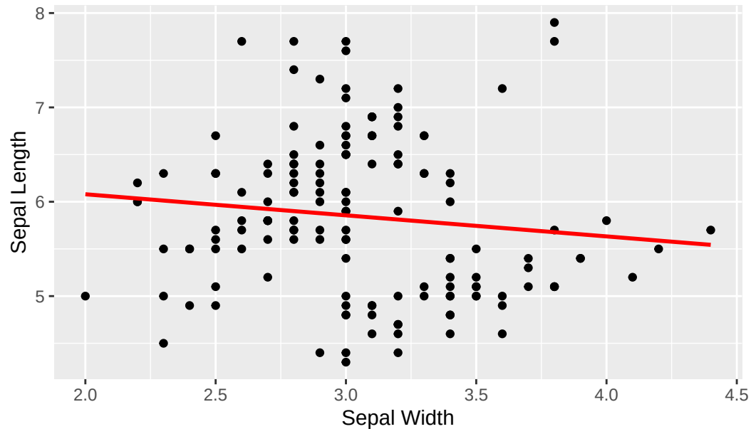
Scatter Plot with the Regression Line
