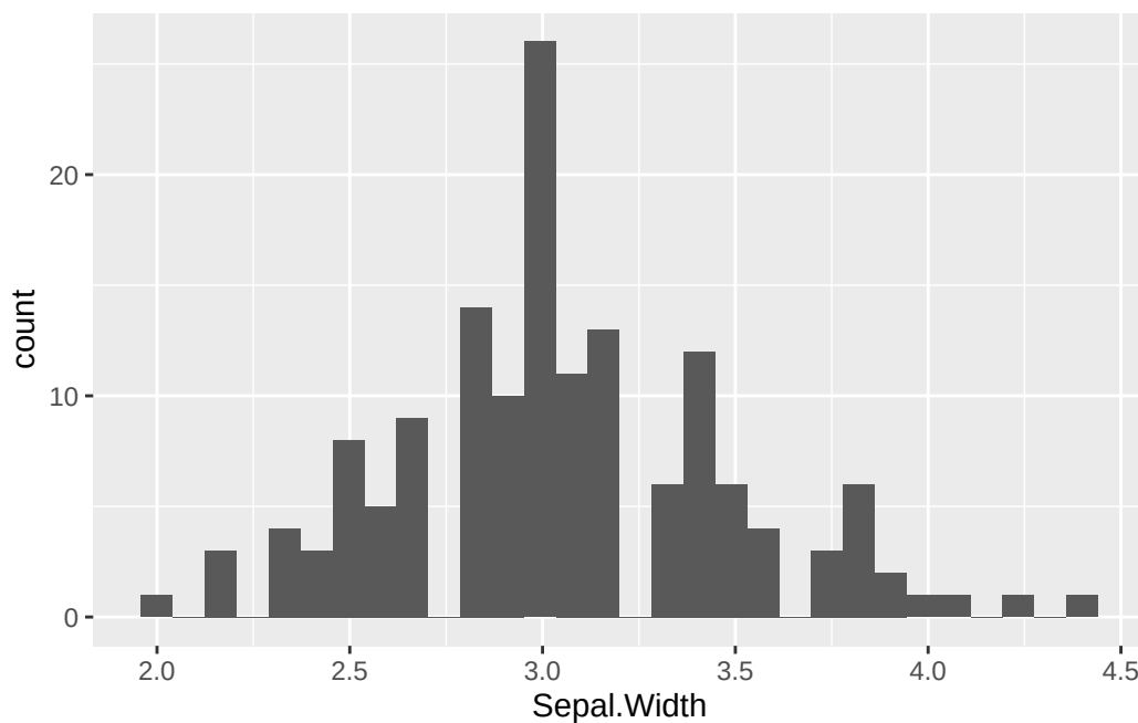
Figure 3.22: ggplot2 Histogram.
