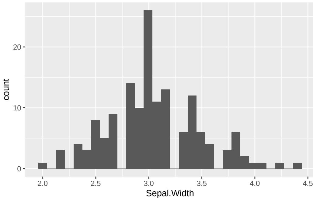
Figure 3.22: ggplot2 Histogram.
