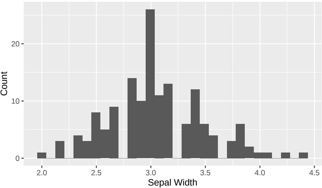
Histogram of Sepal Width
